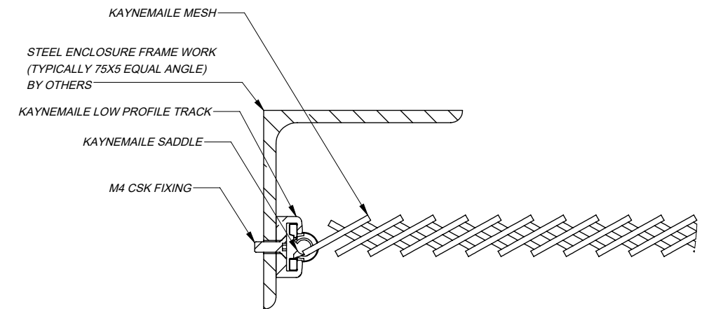
SECTION B-B (CROPPED)
