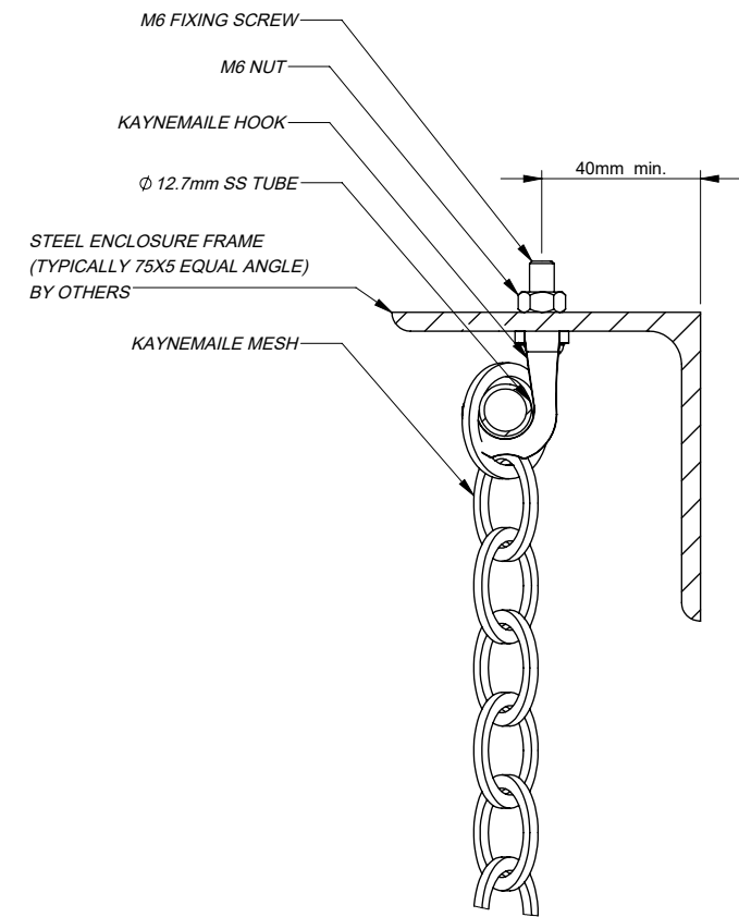
SECTION A-A (CROPPED)
