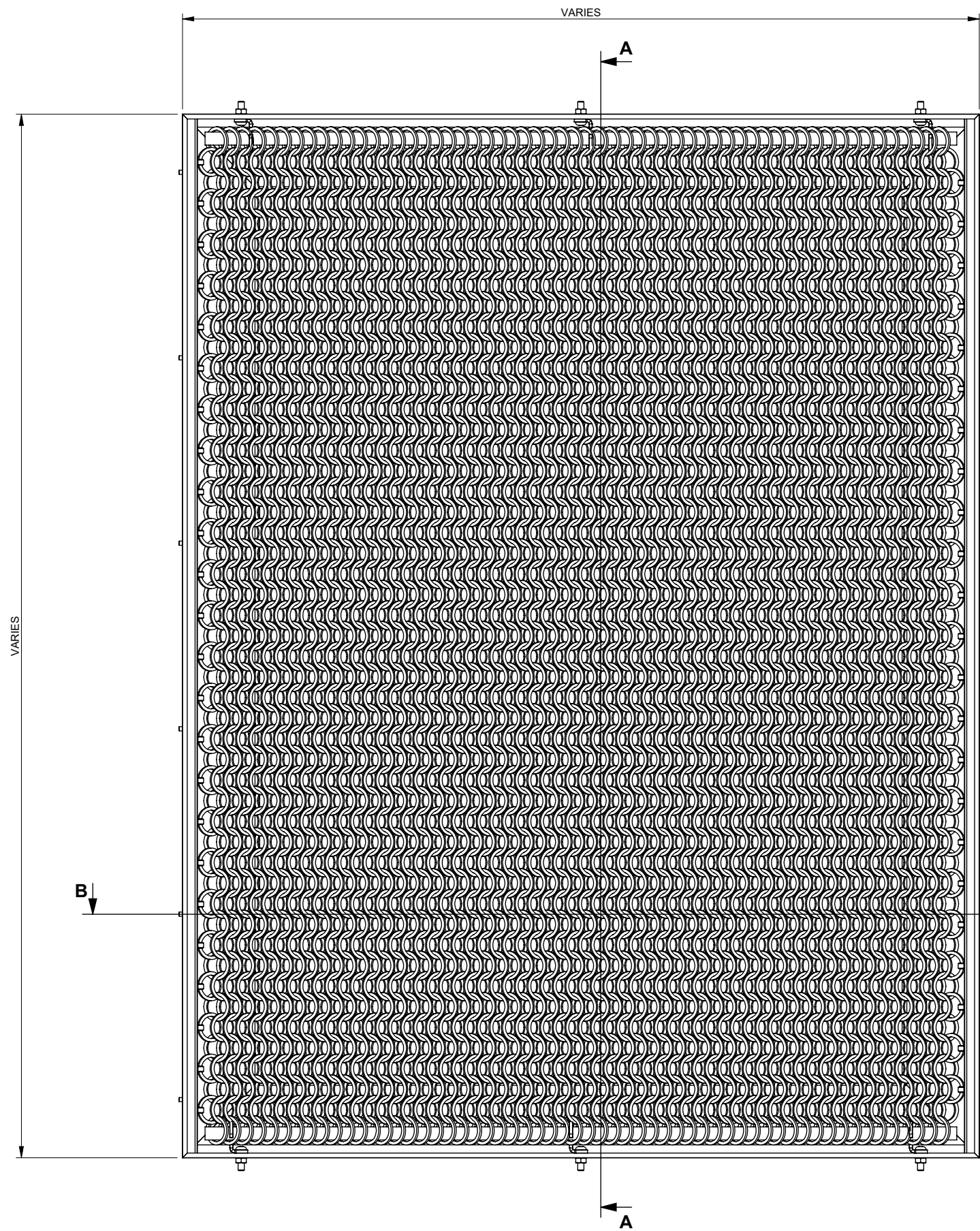
FRONT ELEVATION (TYPICAL EXTERIOR SCREEN)
