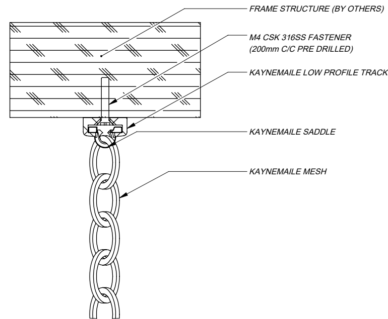
SECTION B-B CROPPED
