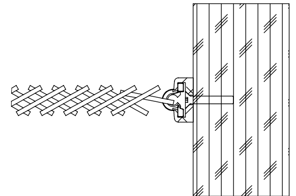
SECTION C-C CROPPED
